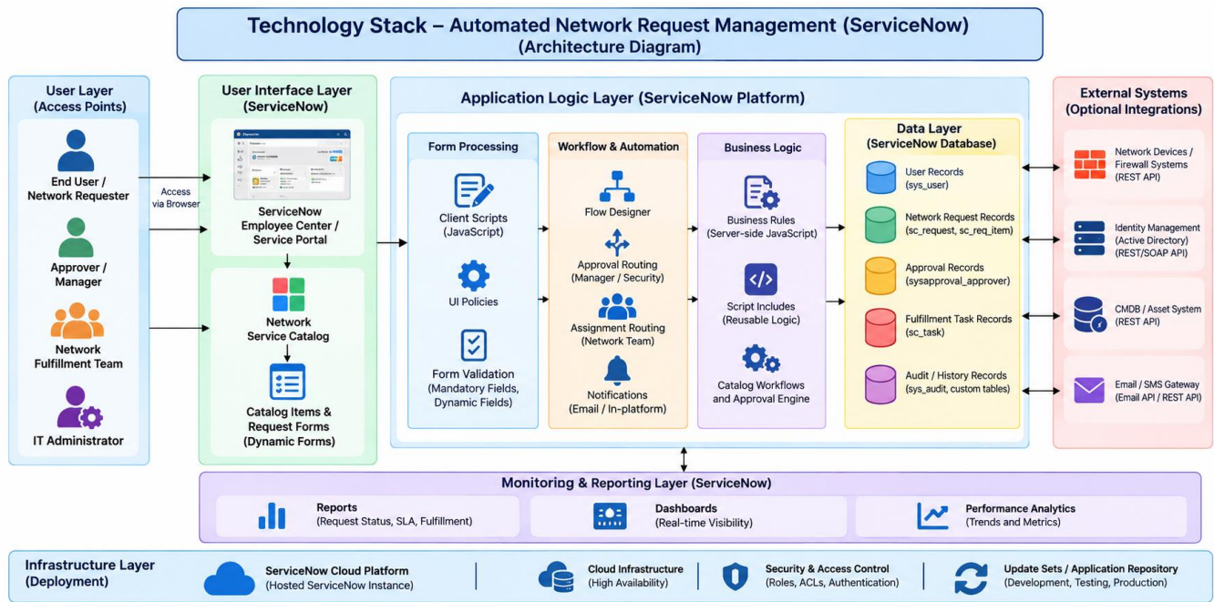
Figure 1: Proposed Technical Architecture – Automated Network Request Management
